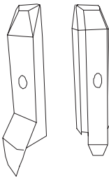
Side Covers
